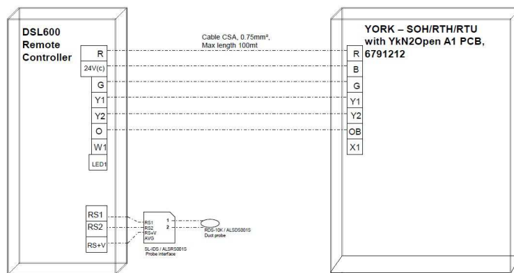
Field control wiring for YORK unit with YkN2Open board
