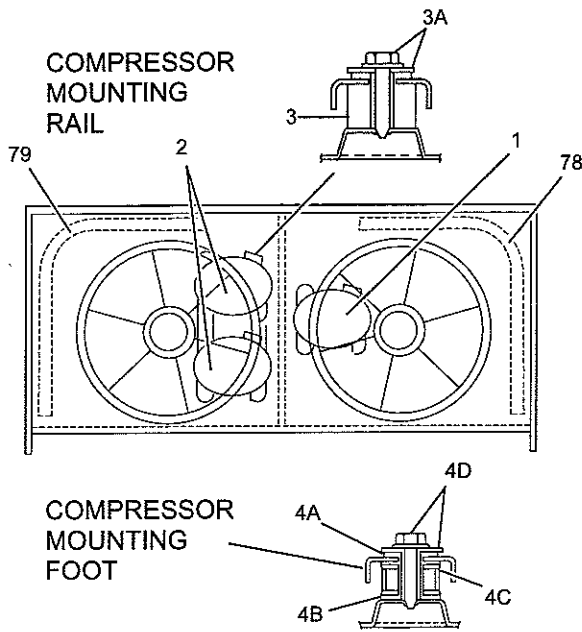
FIG. 2 - COMPRESSOR & COIL SECTION
